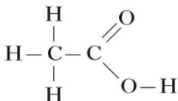
ethanoic acid
